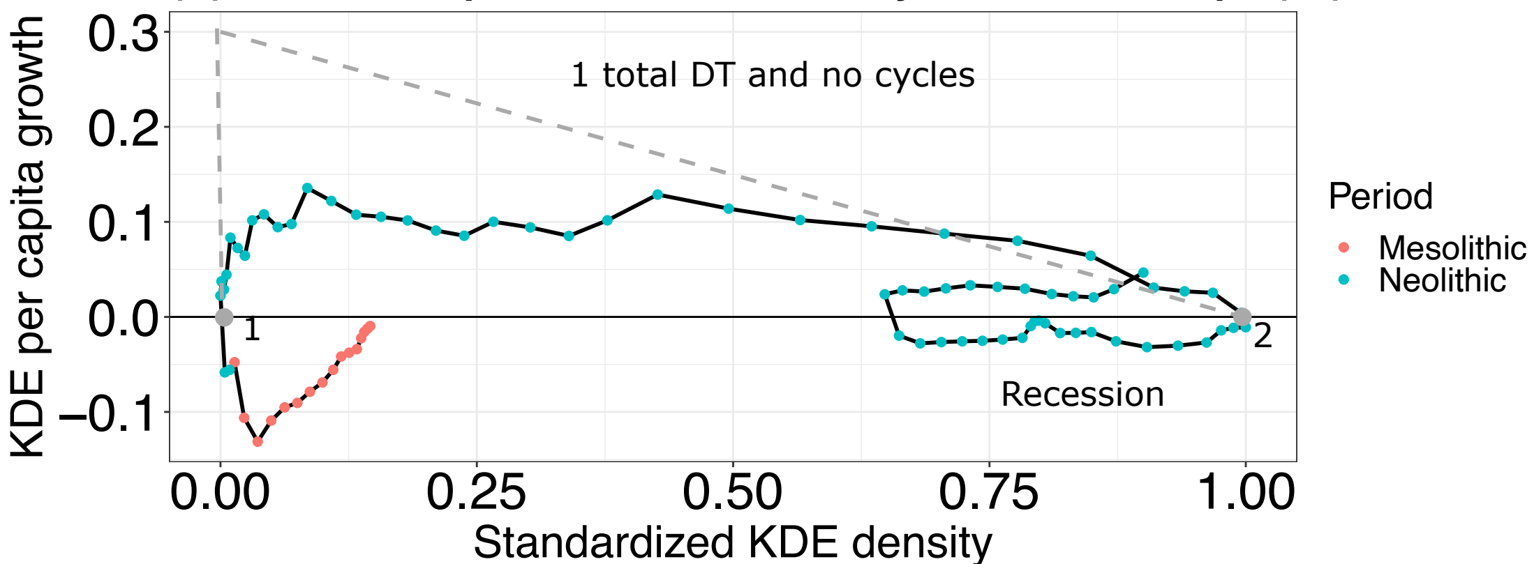
(C) KDE Per Capita Growth vs. Density – West C. Europe (22)
